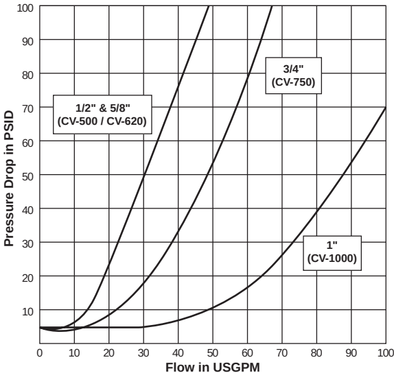
CV Series (1/2", 5/8", 3/4" & 1") Test Fluid: Oil - 200 SUS
