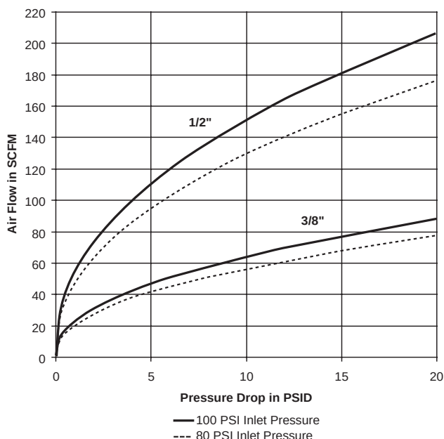
HF Series (3/8" & 1/2" sizes)
