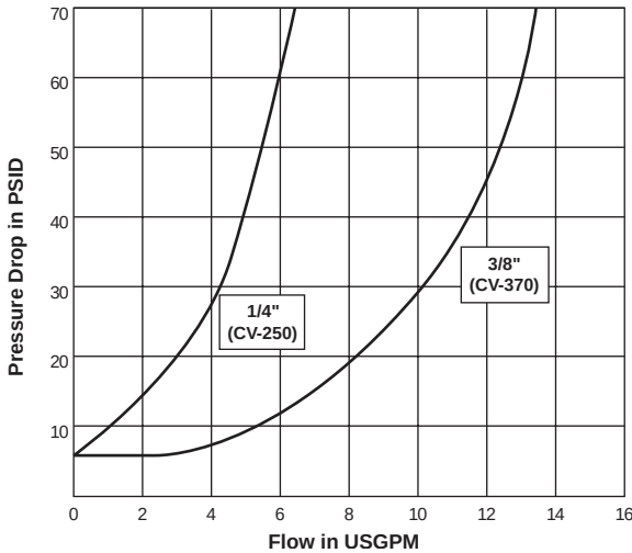
CV Series (1/4" & 3/8") Test Fluid: Oil - 200 SUS
