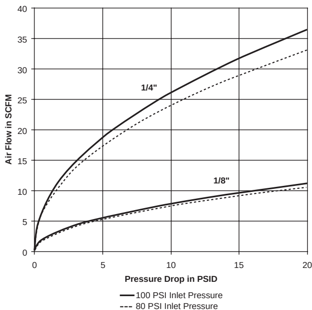
HF Series (1/8" & 1/4" sizes)
